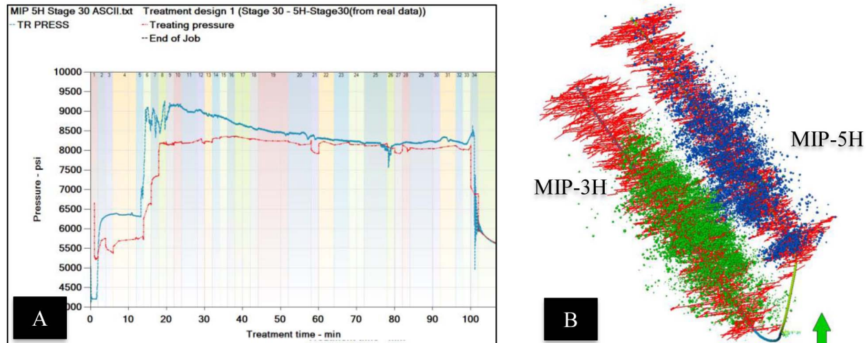
Figure 9—(a) Treating pressure match for stage 30 on MIP-5H. (b) Hydraulic fractures along with microseismic events on MIP-3H and MIP-5H showing good match.
