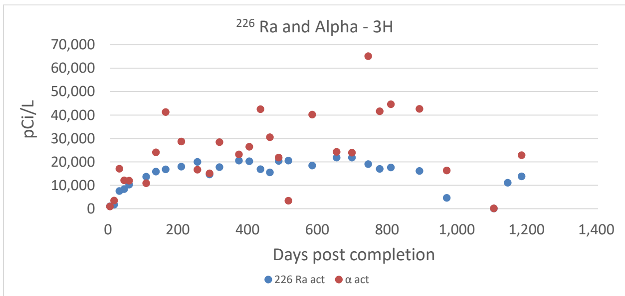
Figure 4.8: The relationship between gross alpha and ^{226}\text{Ra} as a function of time post completion at 3H.
